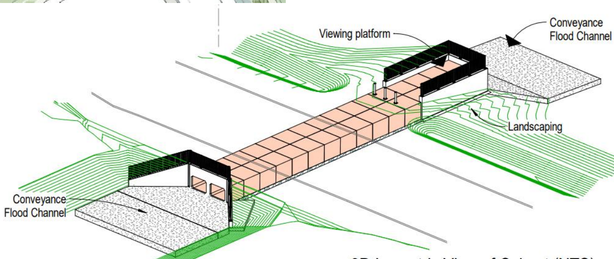
3D Isometric View of Culvert (NTS)
